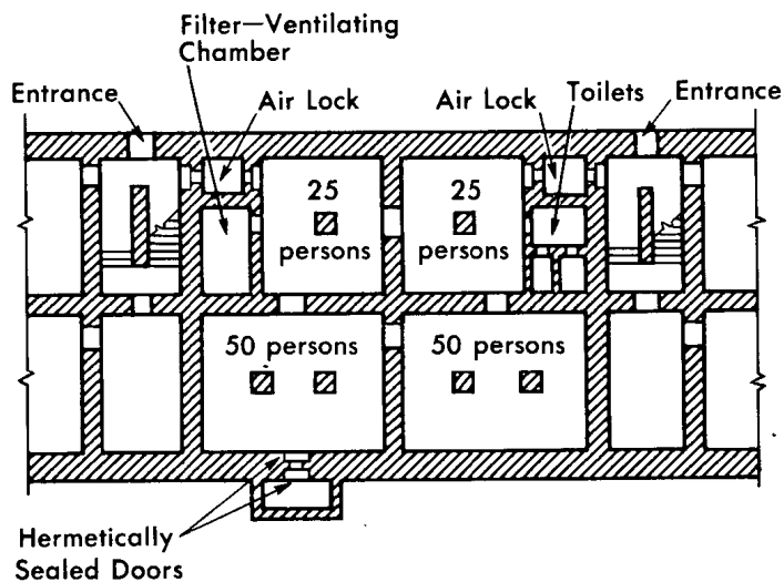
FLOOR PLAN
